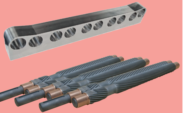
Bearing blocks and peelerollers
