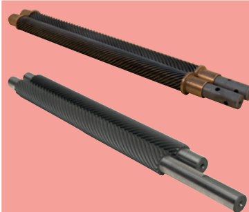
Peelerollers compatible with both Linco and Systemate
